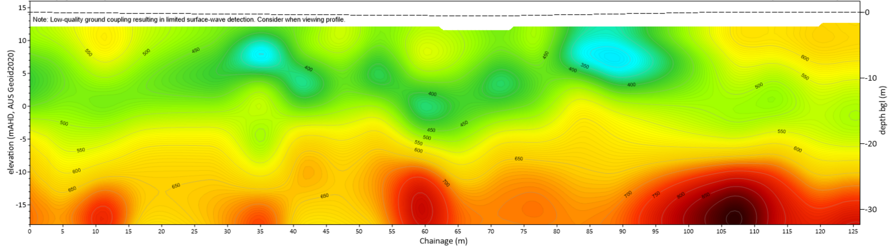
Seismic Line MASW AU-GP 149
